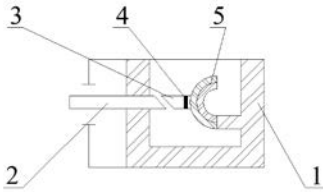
Fig. 5. Fiber-optic vibration sensor wear: 1 – base; 2 – primary fiber; 3 – secondary fiber; 4 – reflective layer; 5 – braided console plate
