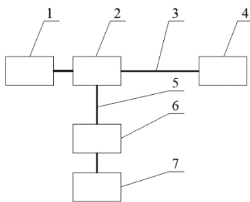
Fig. 1. Block diagram of the measuring system of the wear sensor with Bragg fiber lattice: 1 – radiation source; 2 – splitter; 3 – primary fiber; 4 – fiber with a Bragg lattice that is in contact with the tribo-surface; 5 – secondary fiber; 6 – photodetector; 7 – controller for determining the amount of wear
