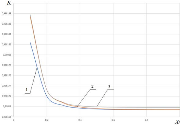
Fig. 4. The relative intensity K depending on the gap x_s between the primary and secondary fibers of artificial sapphire for different wavelengths of optical radiation \lambda , \mu\text{m} : 1 – 0.85; 2 – 1.33; 3 – 1.55
