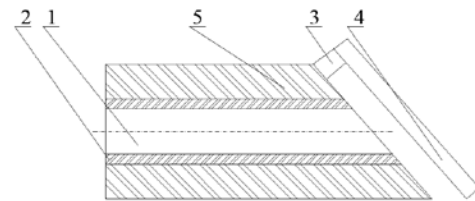
Fig. 3. Vibration wear sensor: 1 – optical fiber; 2 – shell; 3 – console support; 4 – mirror; 5 – basis
