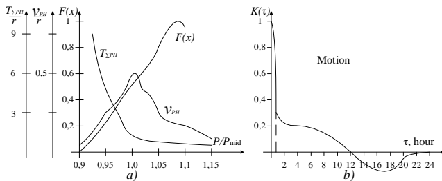
Fig. 6. The results of experimental evaluation load characteristics (a) and the normalized correlation function, designed
