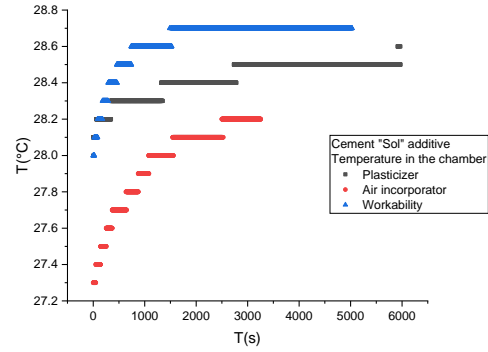
Figure 3. Monitoring of the temperature inside the chamber during the carbonation of the samples.
