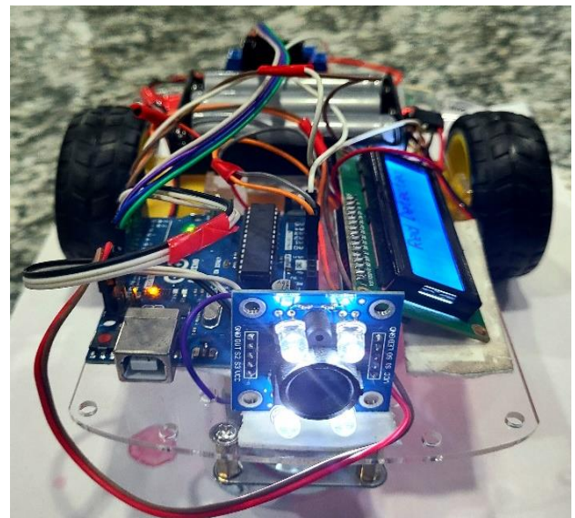
Fig.2. Robot Car.
