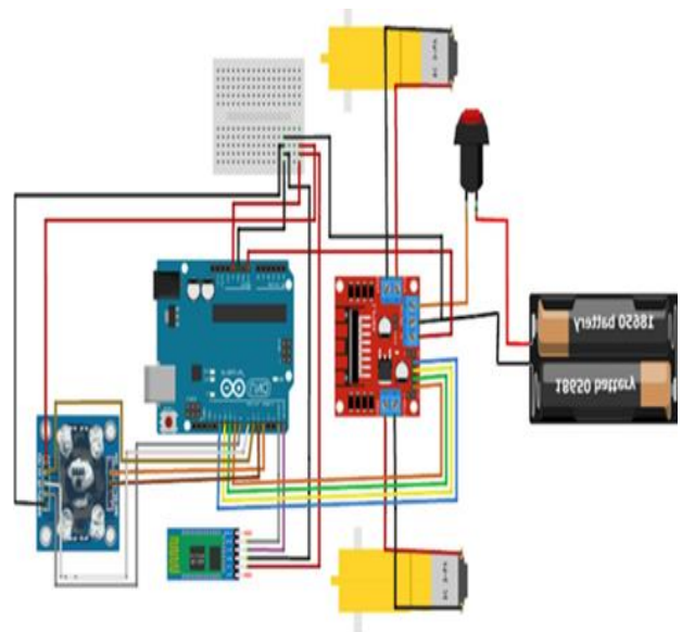
Fig.3. Simulation Diagram.
