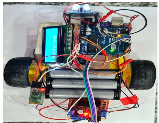
Fig.8. AutoNav Robot Car.
