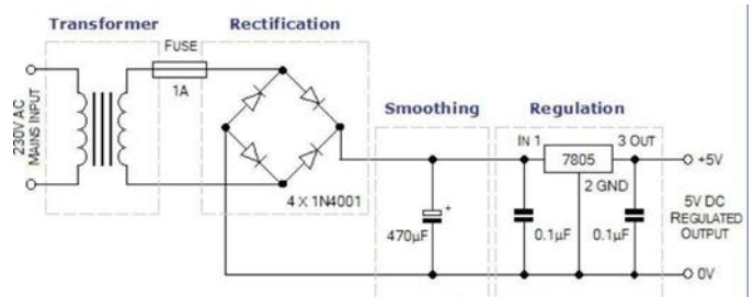
Fig 3.7 Power Supply Unit
