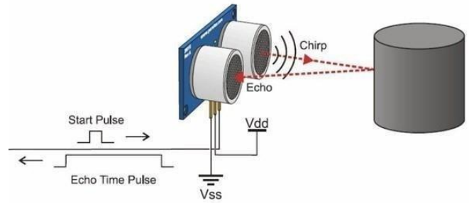
Fig.3.2. Working of ultrasonic sensor
