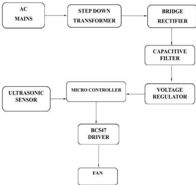
Fig 3.1 Proposed Design
