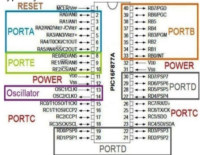
Fig 3.3 Pin details of PIC16F877A microcontroller
