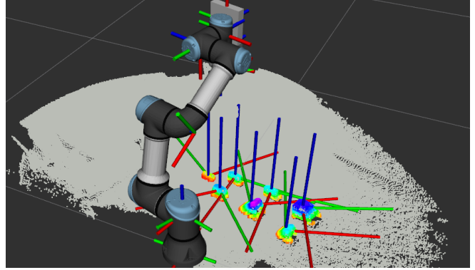
Fig. 5. Real time robot visualization of point cloud data and table scene objects. The centroid of each clustered is associated with a local coordinate frame.
