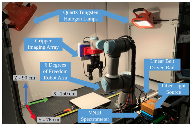
Fig. 1. Spectral benchmarking testbed with architecture to acquire scene hyperspectral datacubes and in-hand spectral data. Note the axes orientations and cell dimensions.
