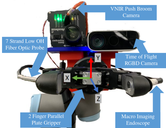
Fig. 2. Multi-modal perception setup for sensing both spatial-spectral characteristics of total workspace and in-hand. NB: Z-axis is perpendicular, coming out of the page.
