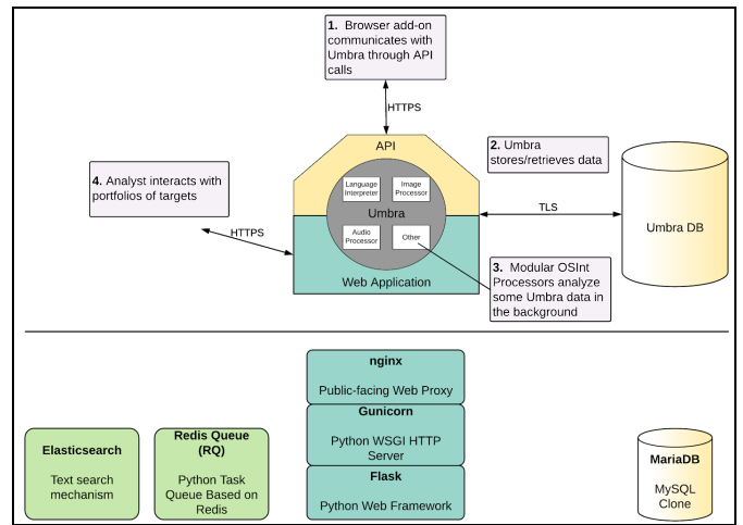
Fig. 1. Umbra usage and software stack.
