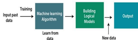
Fig. 2. Machine Learning
