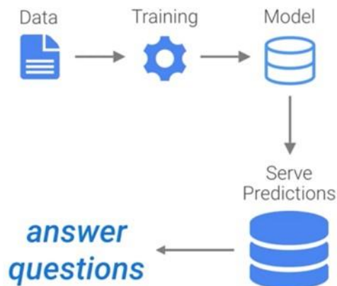
Fig. 1. Machine Learning
