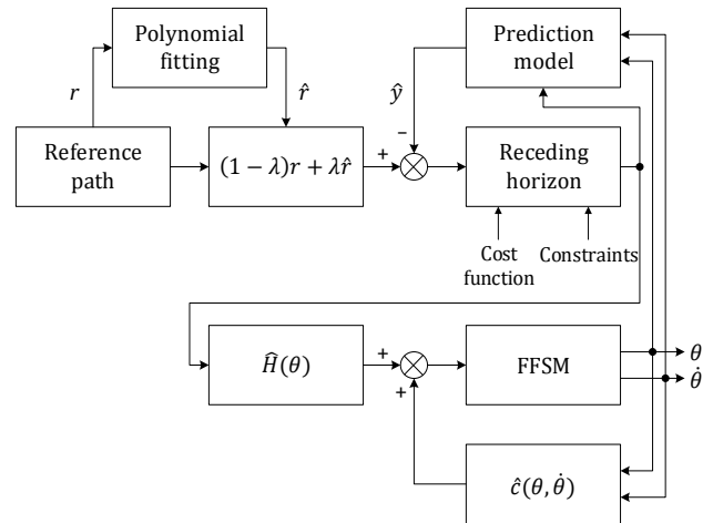
Fig. 3. Block diagram of the proposed approach
