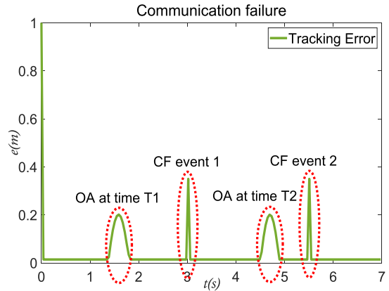
Fig. 6. Time evolution of the tracking error
