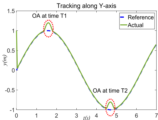
Fig. 5. Time evolution of FFSM tracking along Y-axis
