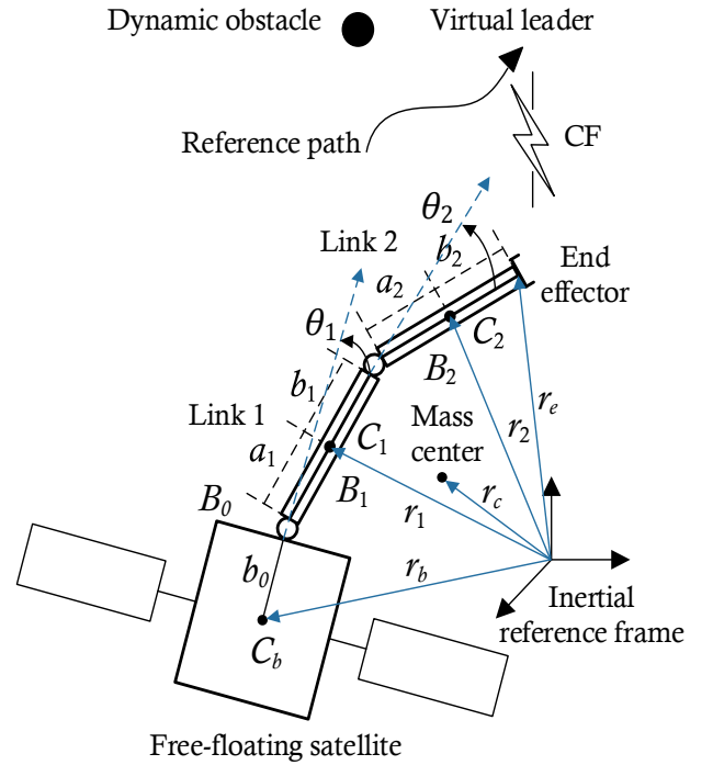
Fig. 1. FFSM scheme with moving obstacles
